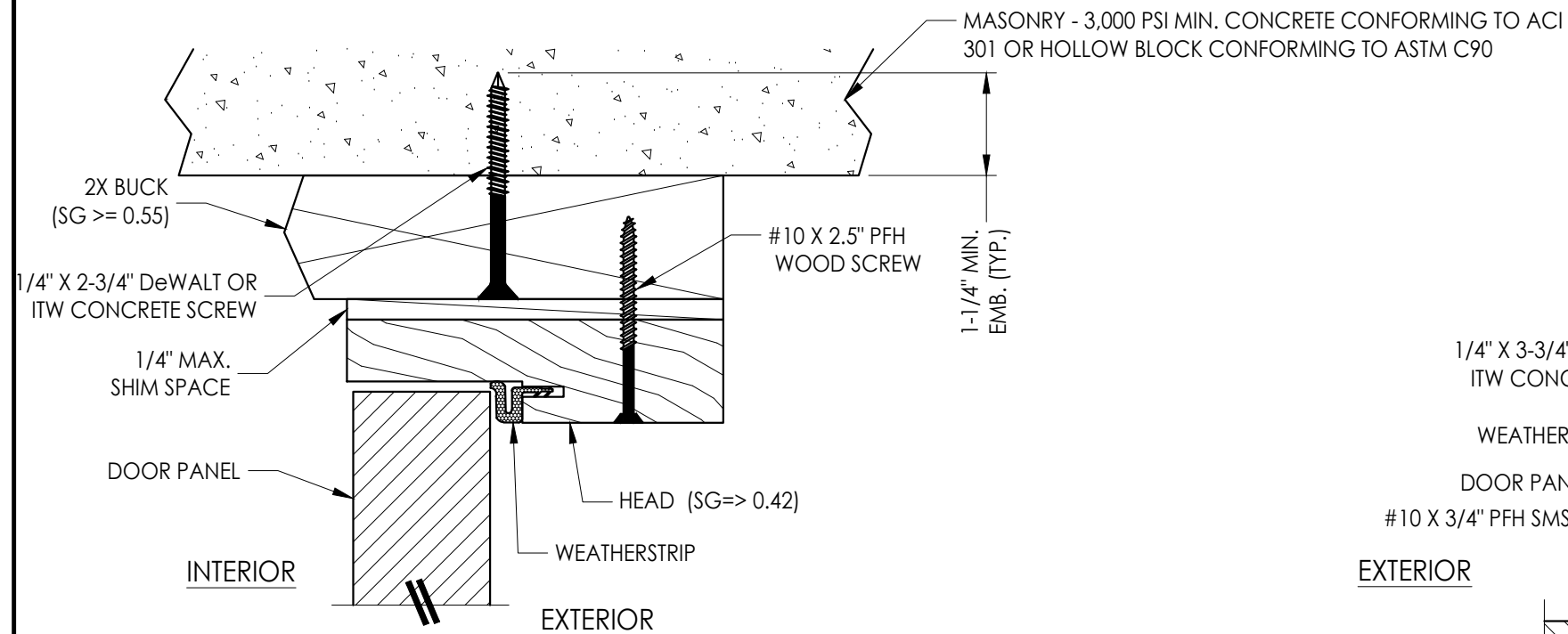
1 4 VERTICAL CROSS SECTION
