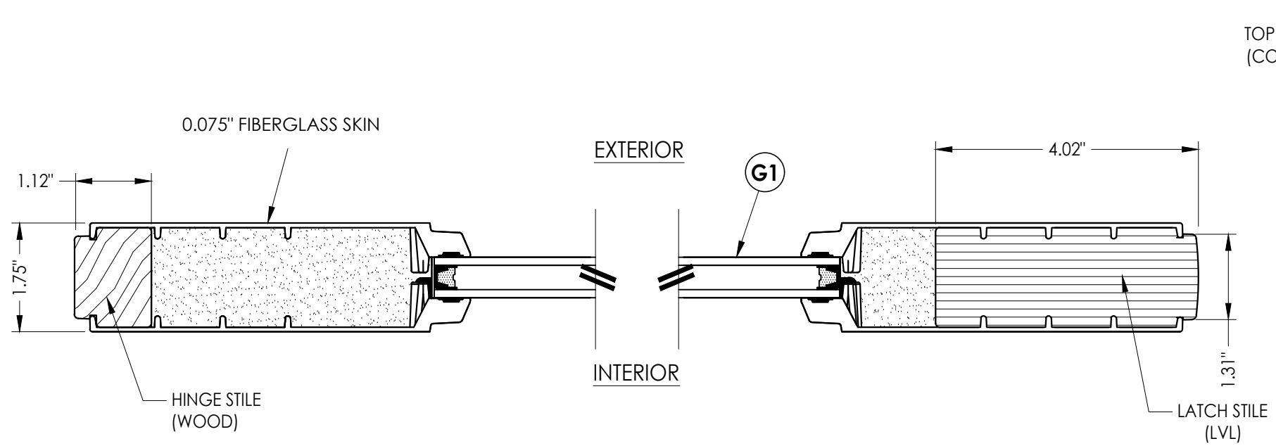
1 3 HORIZONTAL CROSS SECTION
